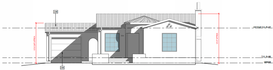
EXISTING FRONT ELEVATION | 4 SCALE: 1/4" = 1'-0"
