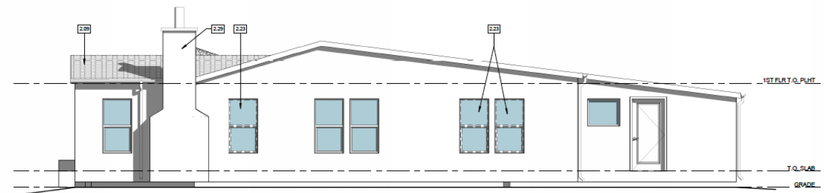
EXISTING RIGHT ELEVATION | 2 SCALE: 1/4" = 1'-0"
