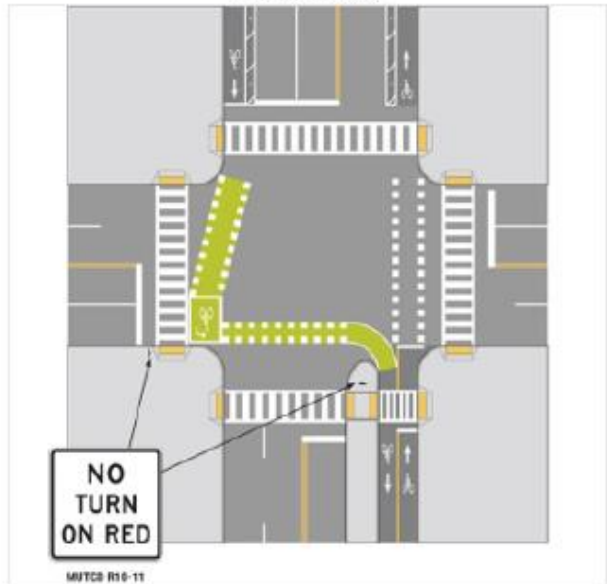
MassDOT provides example intersection configurations to transition between one-way and two-way cycle tracks. Source: MassDOT Separated Bike Lane Planning and Design Guide
