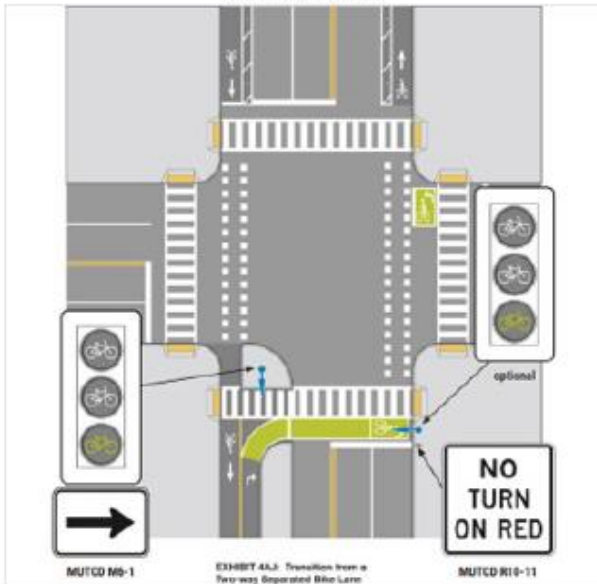
MassDOT provides example intersection configurations to transition between one-way and two-way cycle tracks. Source: MassDOT Separated Bike Lane Planning and Design Guide
