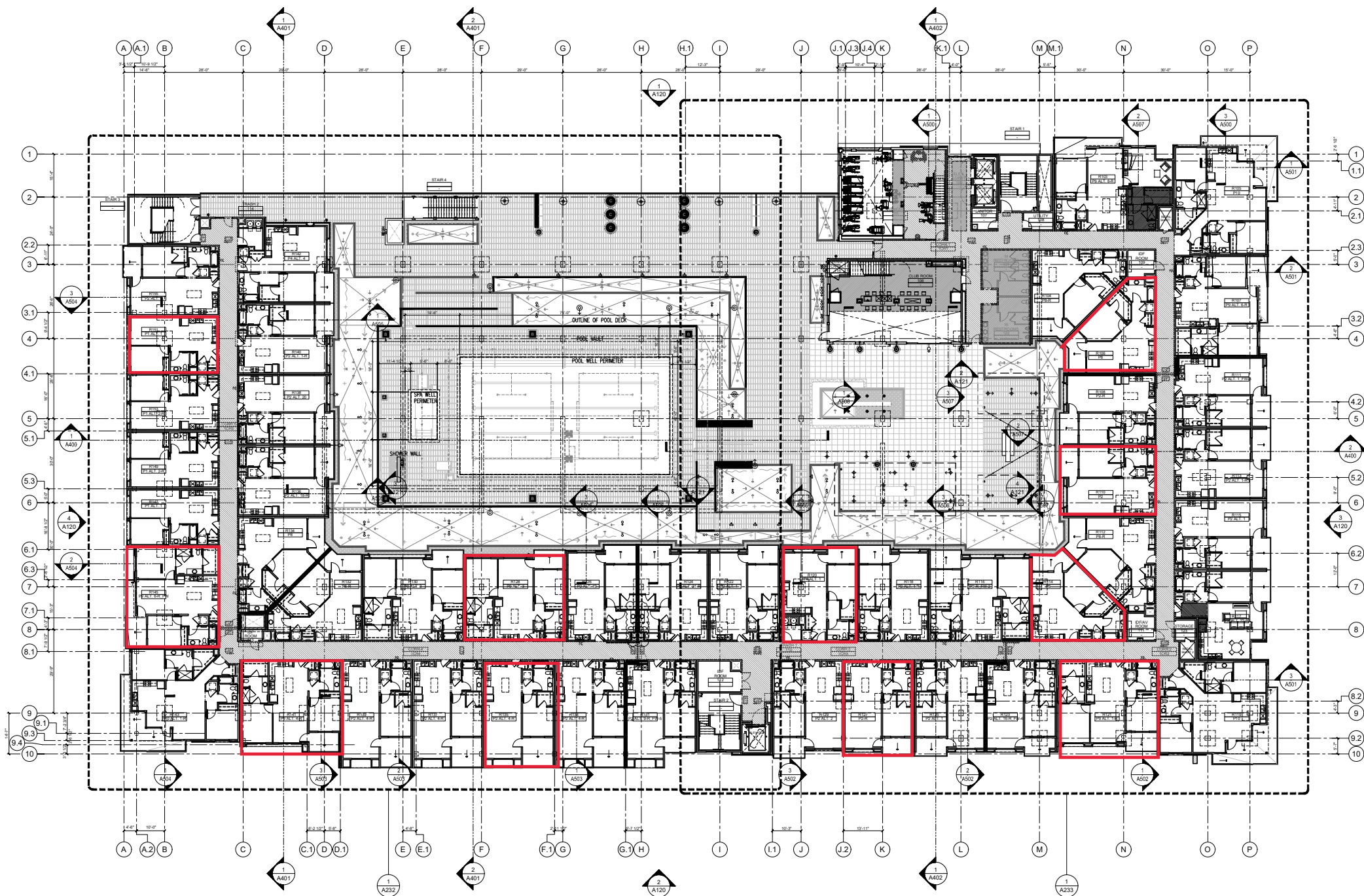
LAWRENCE STATION - BUILDING B R1 PODIUM FLOOR PLAN
