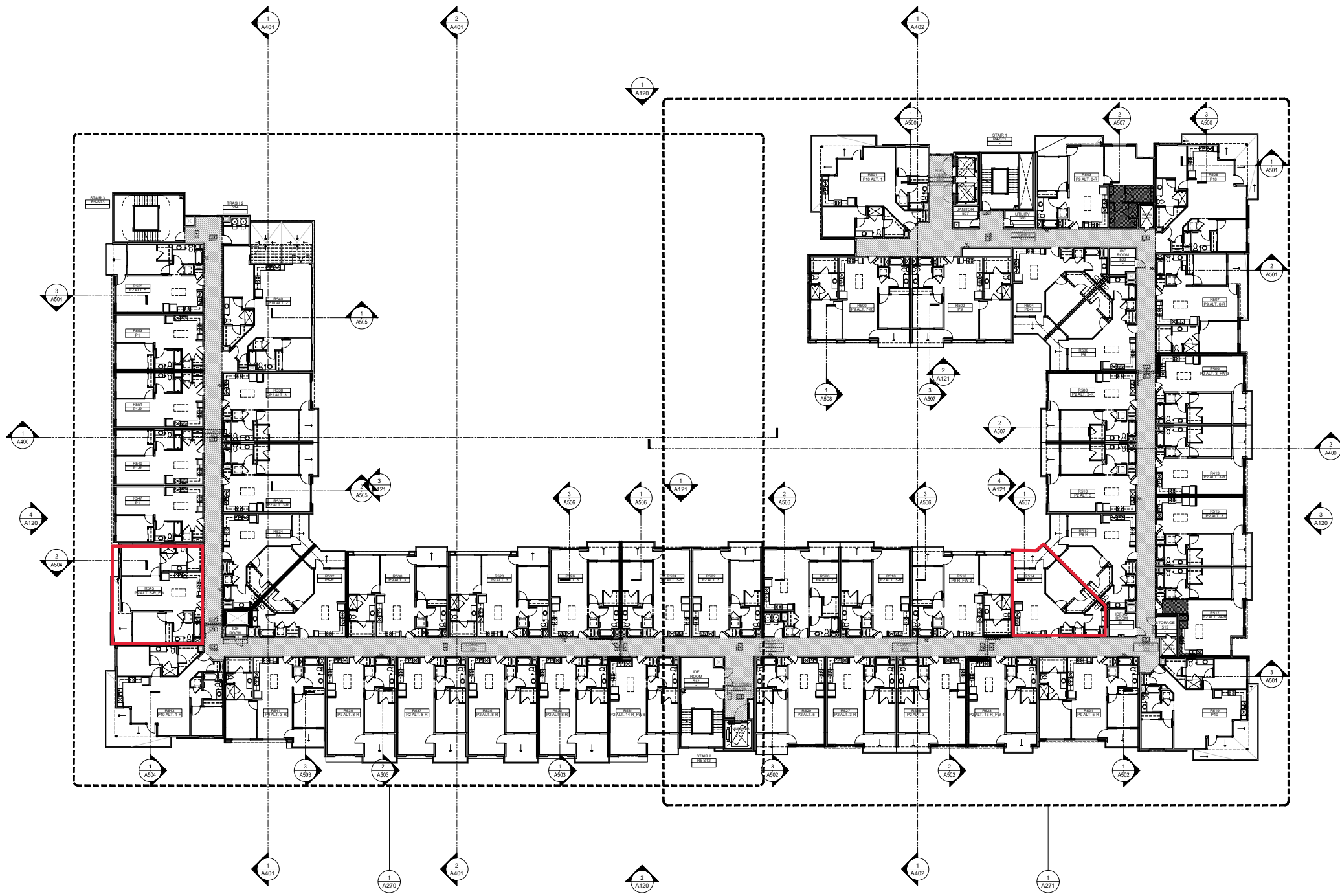
LAWRENCE STATION - BUILDING B R5 FLOOR PLAN
