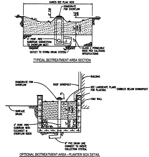
TYPICAL BIOTREATMENT AREA - PLANTER BOX DETAIL
