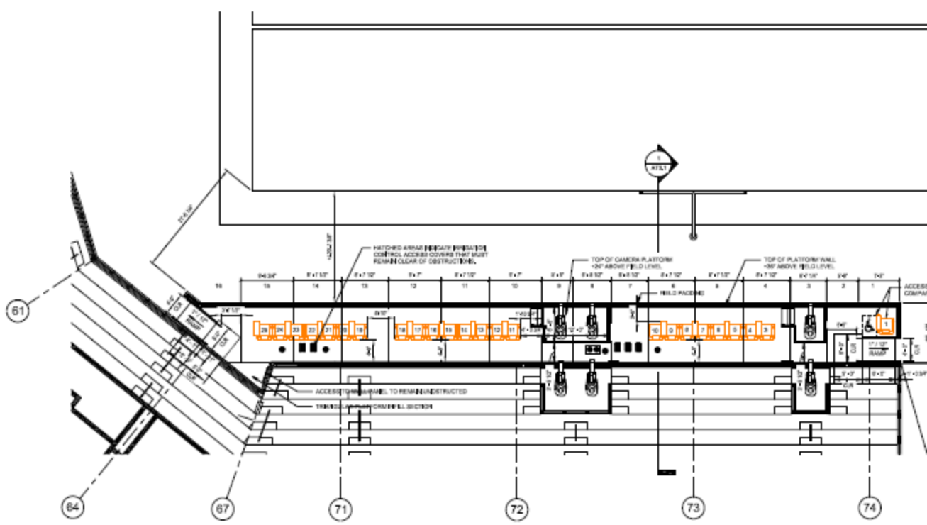
② 100 LEVEL FIELD CLUB PLAN - SOUTH 1/8" = 1'-0"
