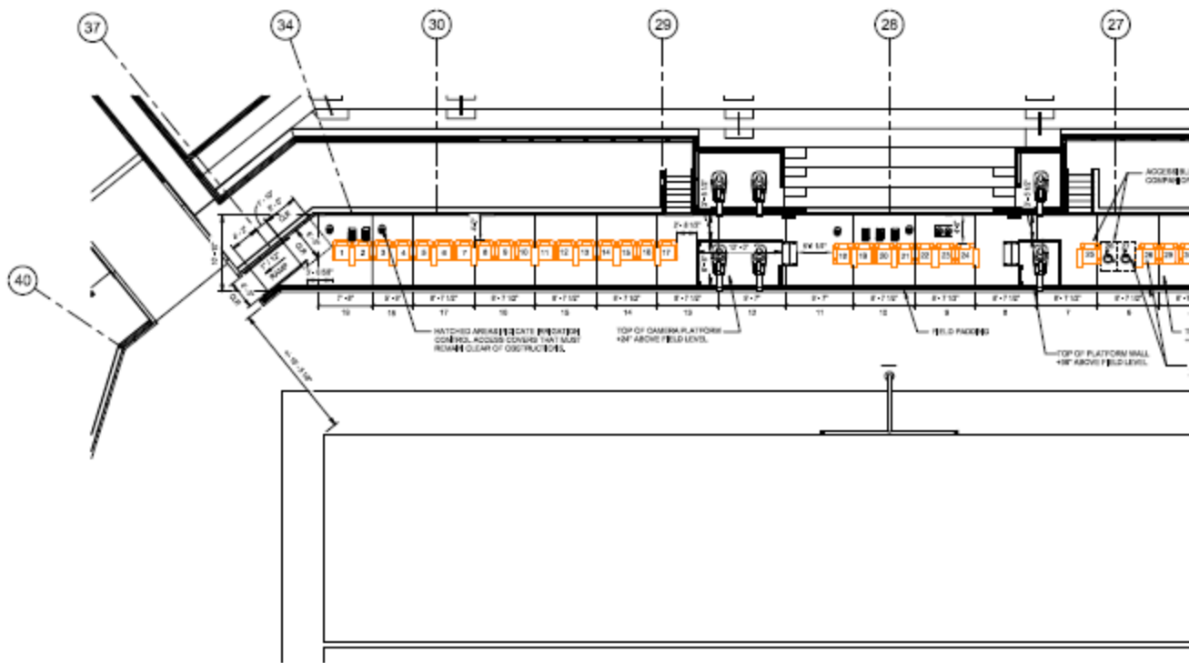
① 100 LEVEL FIELD CLUB PLAN - NORTH 1/8" = 1'-0"
