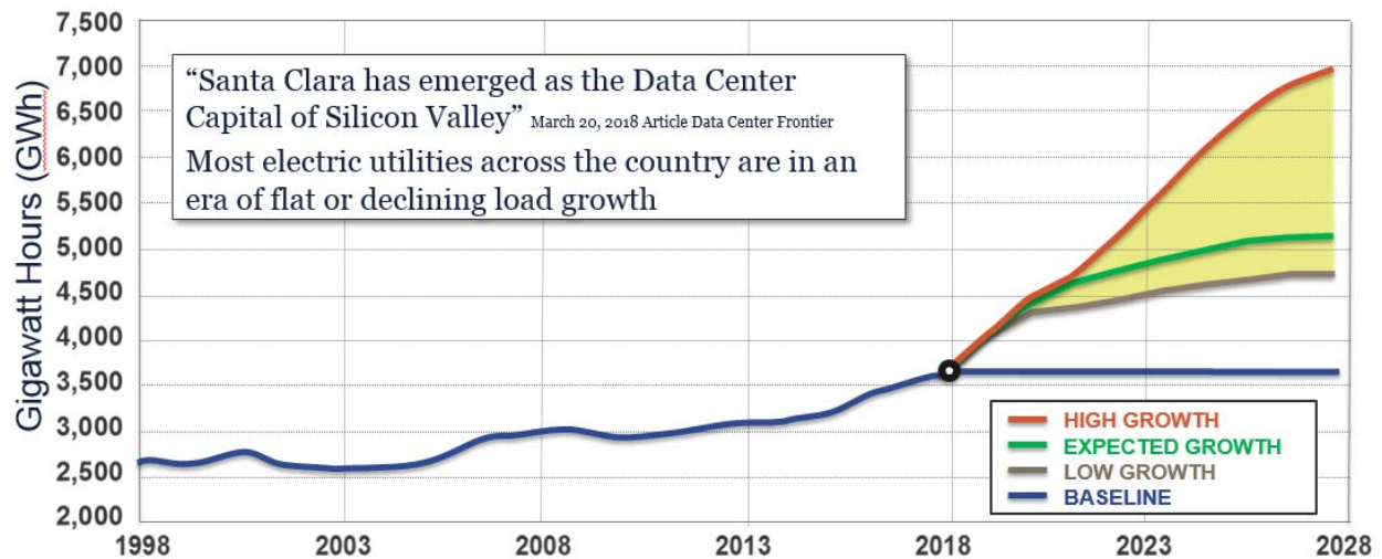
Figure 2-2 SVP Load Growth
