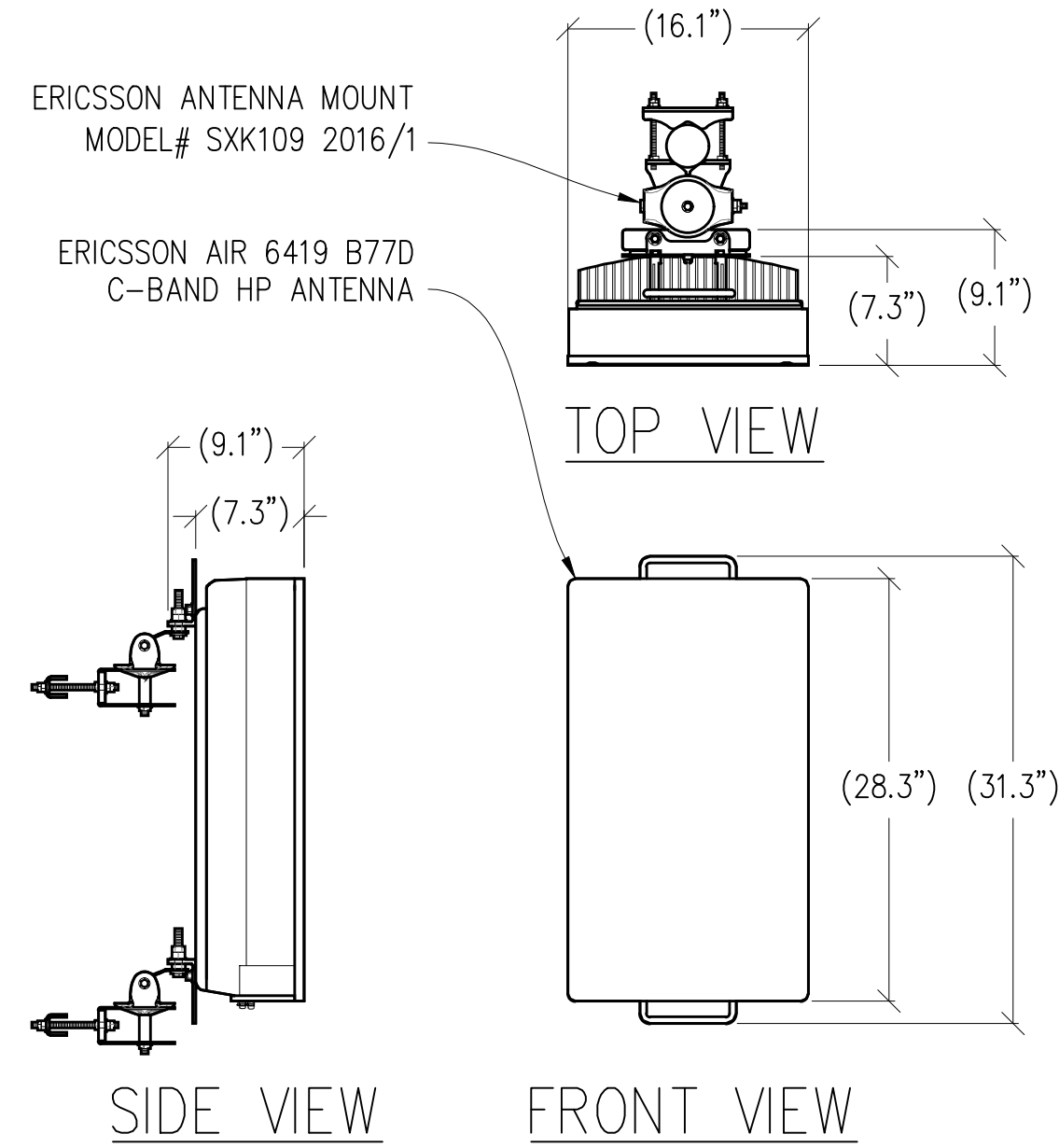
4 ANTENNA DETAIL 1"=1'-0" MAX WEIGHT: 64 LBS
