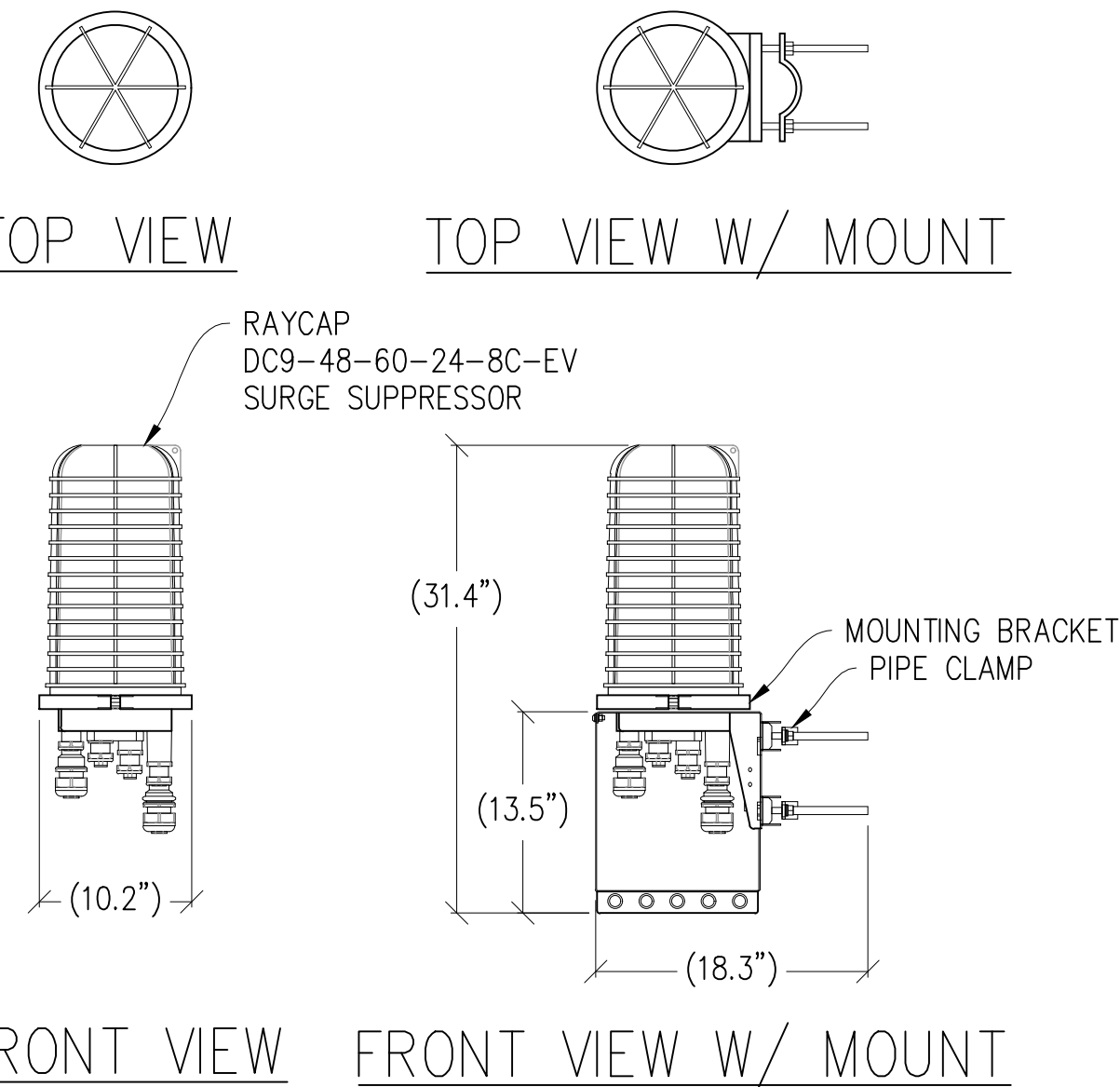
8 SURGE SUPPRESSOR DETAIL 1"=1'-0" MAX WEIGHT = 26.2 LBS
