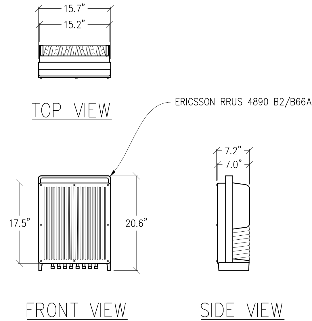
6 RADIO 4890HP DETAIL 1"=1'-0" MAX WEIGHT: 68 LBS
