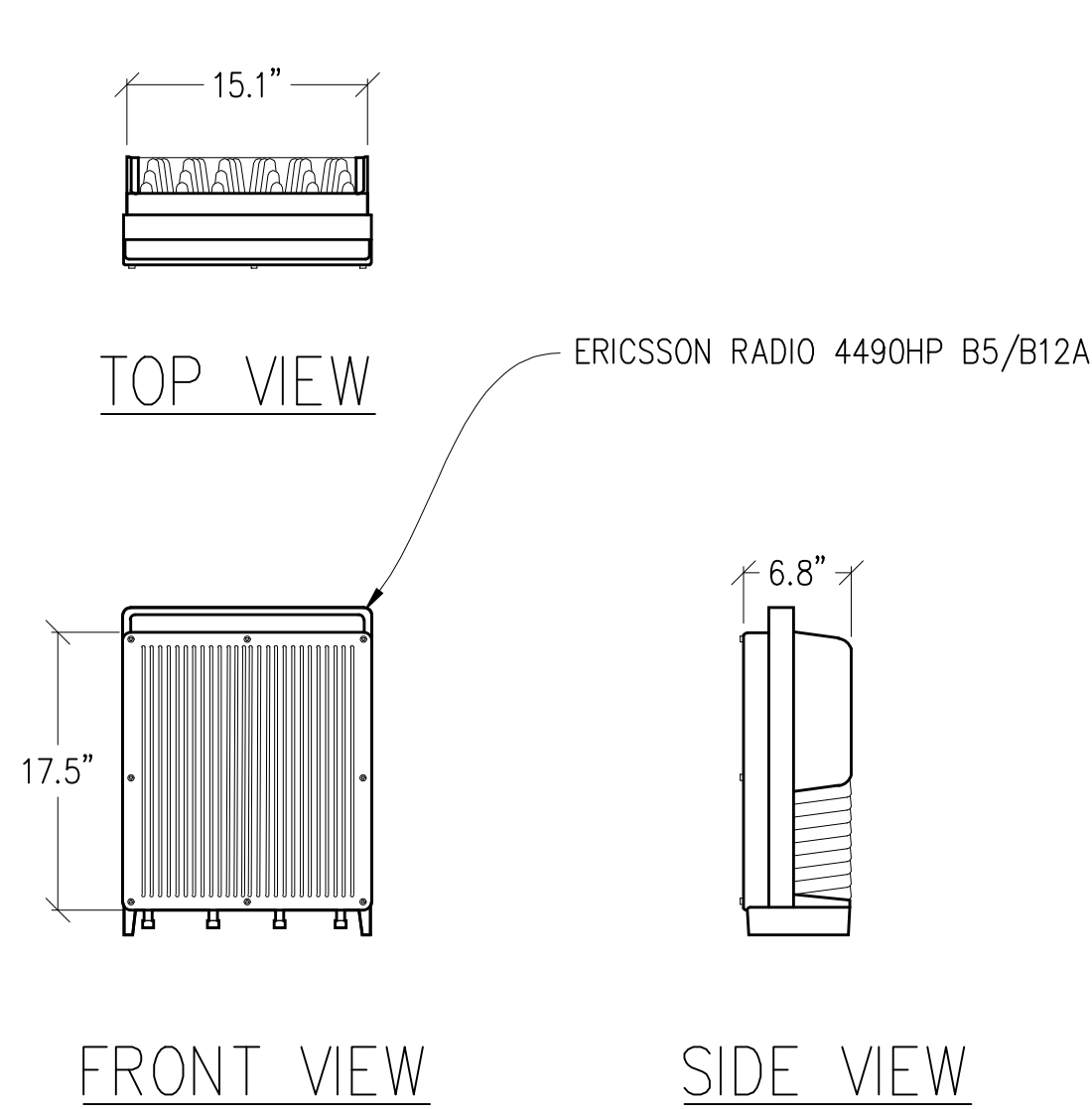
5 RADIO 4490HP DETAIL 1"=1'-0" MAX WEIGHT: 68 LBS
