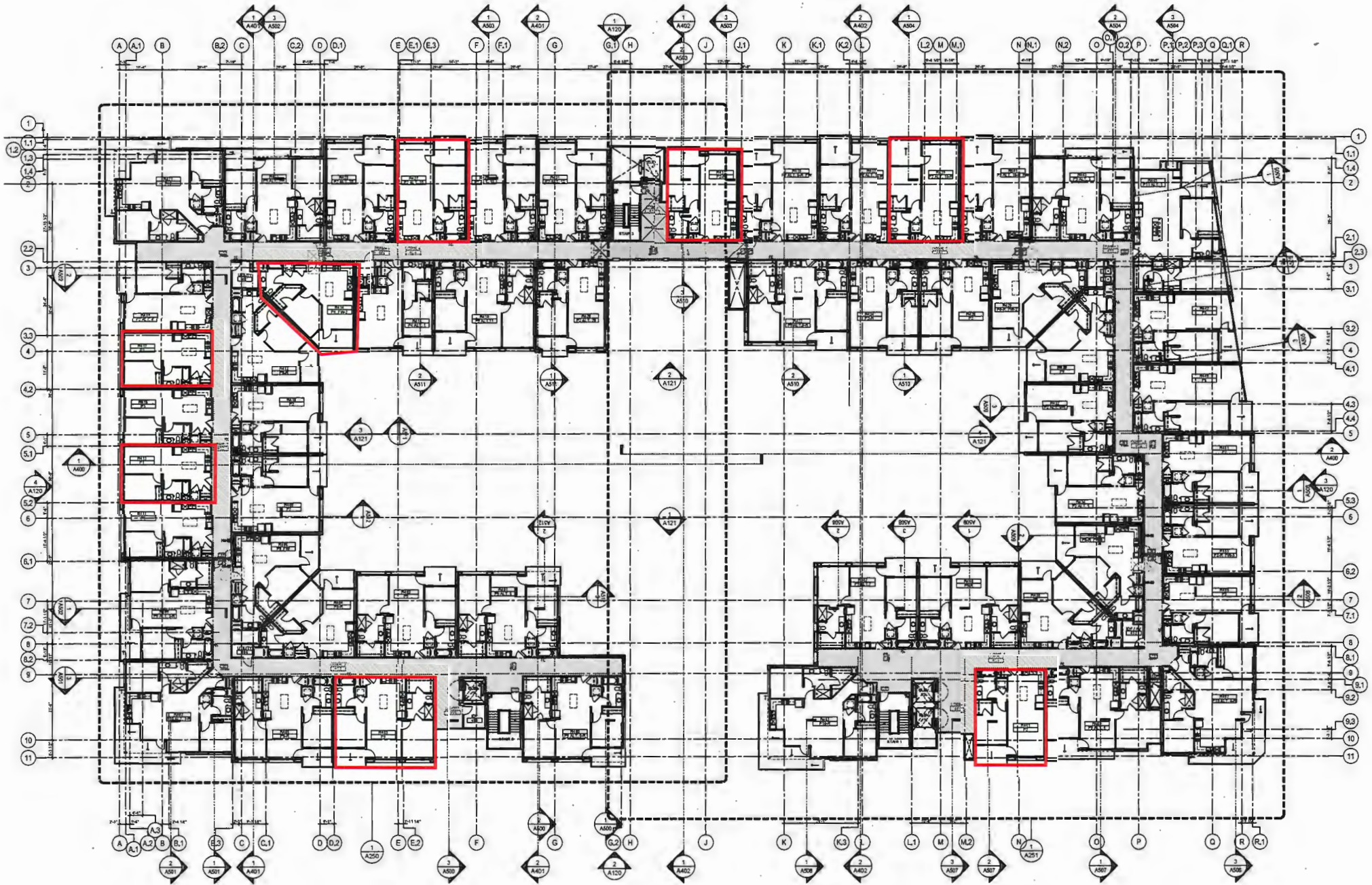
LAWRENCE STATION - BUILDING A R4 FLOOR PLAN
