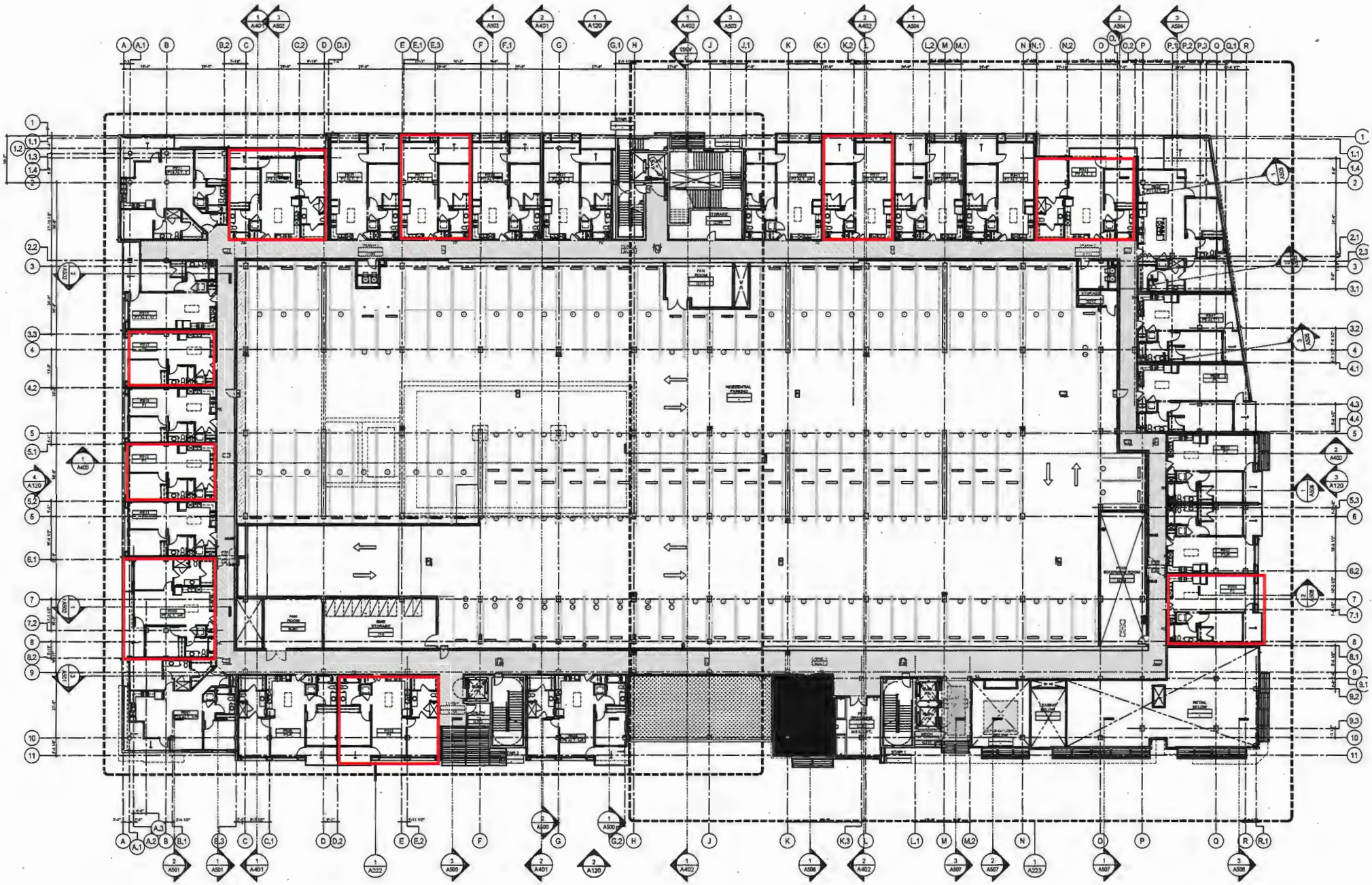
LAWRENCE STATION - BUILDING A G2 FLOOR PLAN
