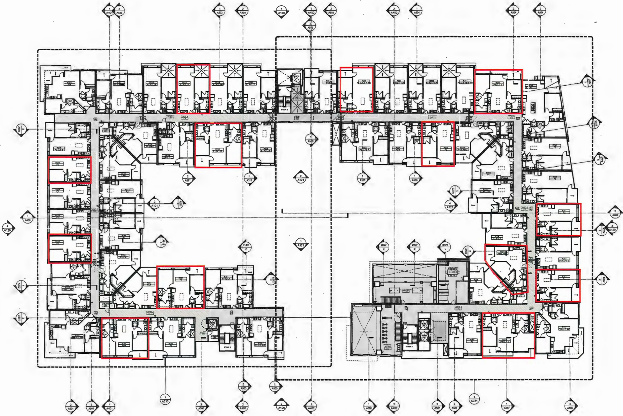
LAWRENCE STATION - BUILDING A R2 FLOOR PLAN
