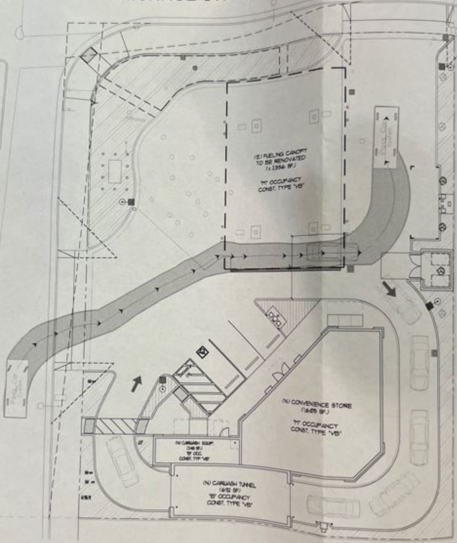
1 CAR PATH SITE PLAN SCALE: 1" = 10'-0"
