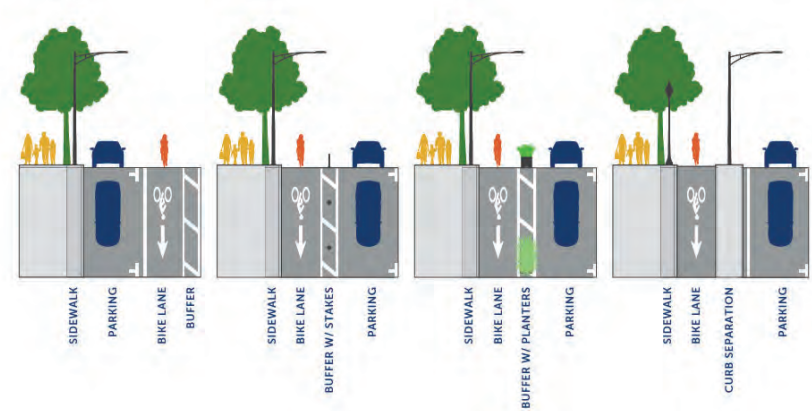
Figure 11: Bicycle Lane Protection Options
