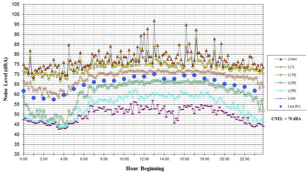
Noise Levels at Noise Measurement Site LT-3 Along Northeast Property Line, ~50 Feet South of Coleman Ave Centerline Saturday, March 18, 2017
