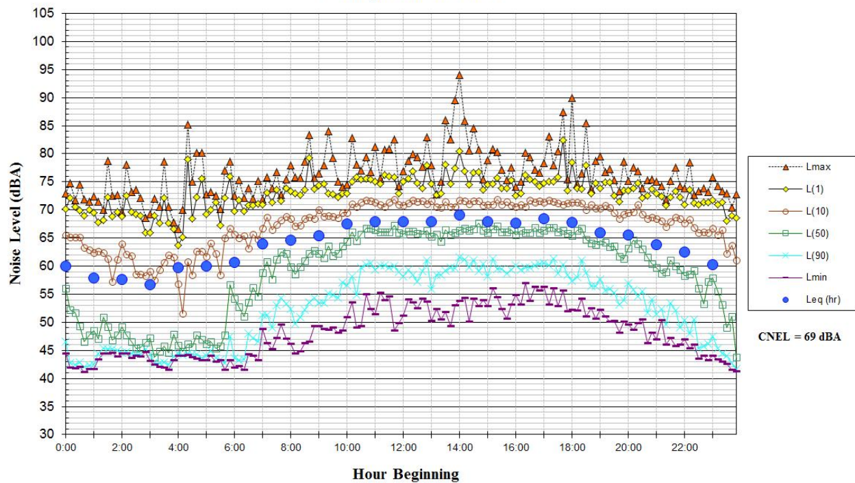
Noise Levels at Noise Measurement Site LT-3 Along Northeast Property Line, ~50 Feet South of Coleman Ave Centerline Sunday, March 19, 2017
