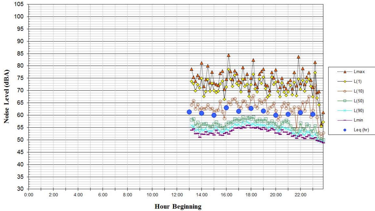
Noise Levels at Noise Measurement Site LT-1 Along Northwest Property Line, ~30 Feet Southeast of Brokaw Road Centerline Thursday, March 16, 2017
