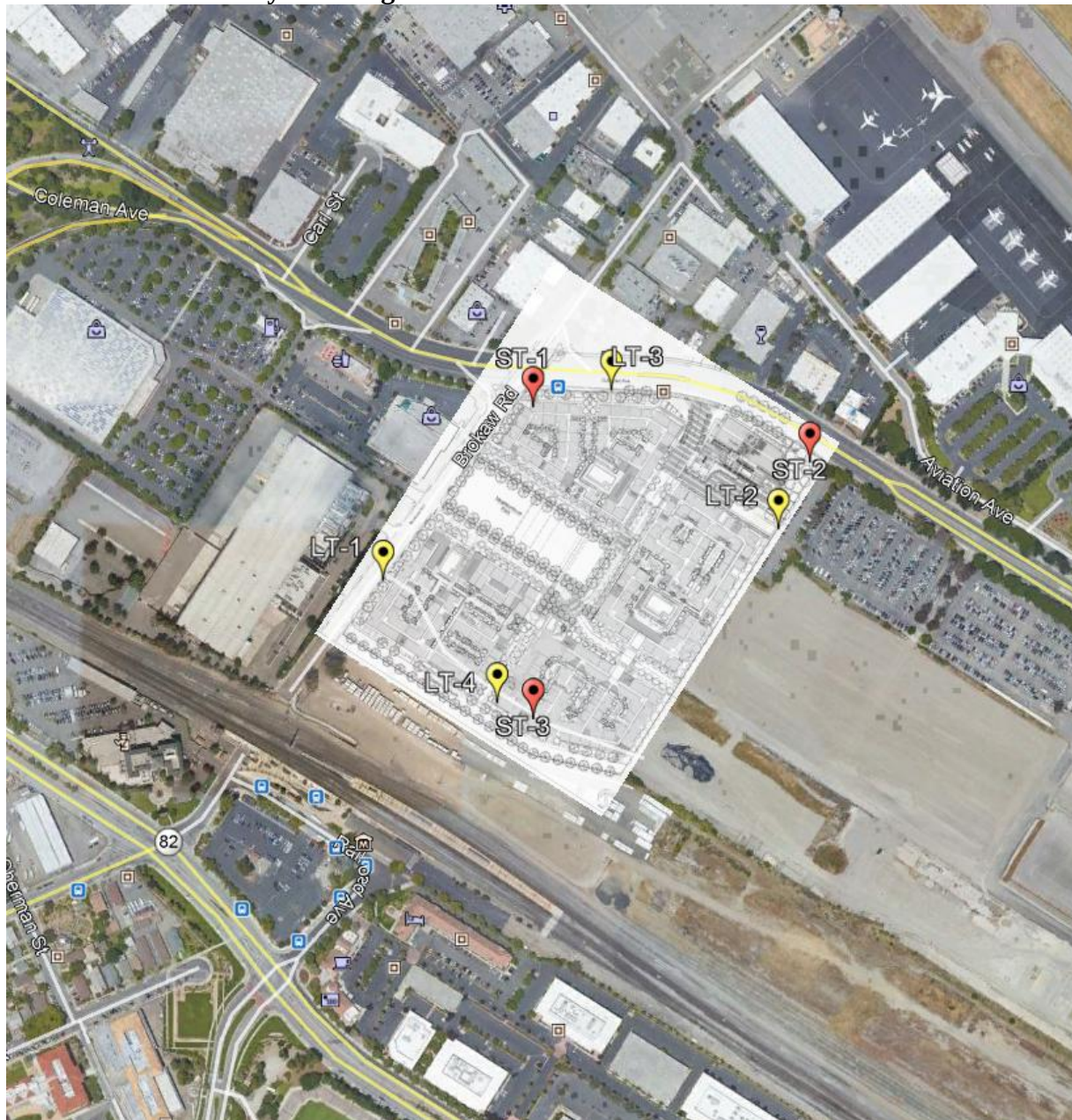
FIGURE 1 Gateway Crossings Noise Measurement Locations
