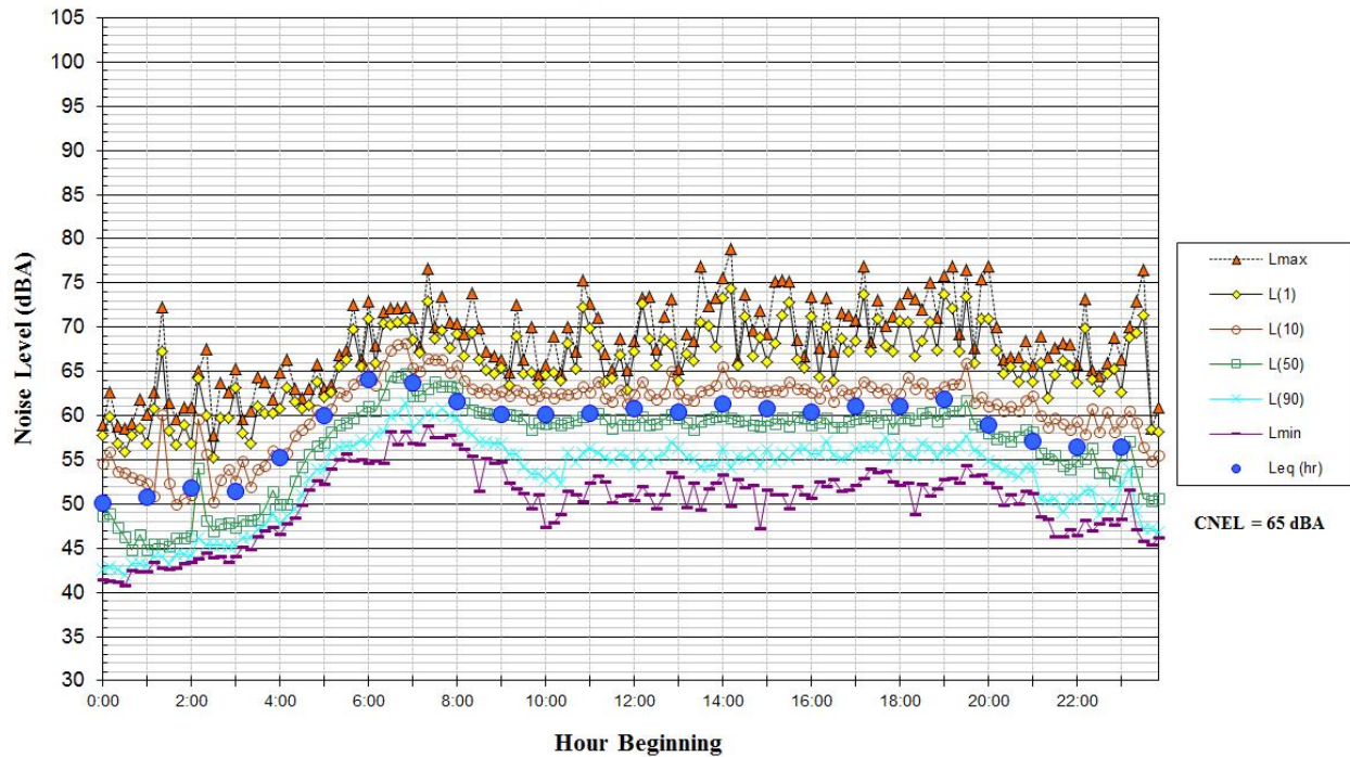
Noise Levels at Noise Measurement Site LT-2 Along Southeast Property Line, ~290 Feet Southwest of Coleman Ave Centerline Friday, March 17, 2017
