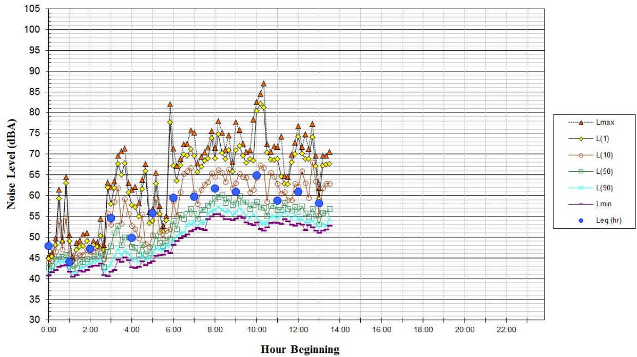
Noise Levels at Noise Measurement Site LT-4 Near Southwest Property Line, ~510 Feet Southeast of Brokaw Road Centerline Monday, March 20, 2017
