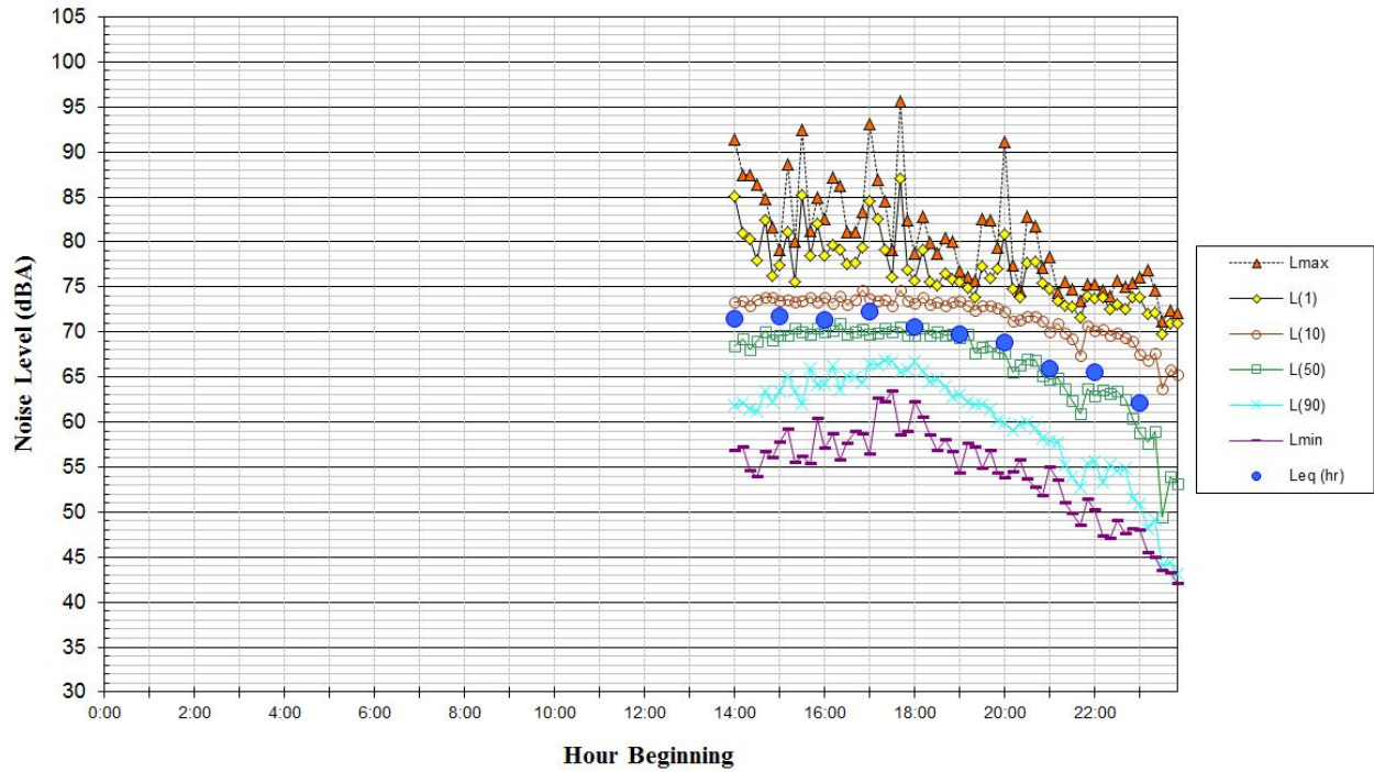
Noise Levels at Noise Measurement Site LT-3 Along Northeast Property Line, ~50 Feet South of Coleman Ave Centerline Thursday, March 16, 2017
