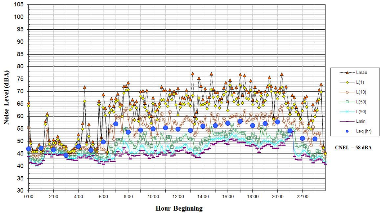
Noise Levels at Noise Measurement Site LT-4 Near Southwest Property Line, ~510 Feet Southeast of Brokaw Road Centerline Sunday, March 19, 2017
