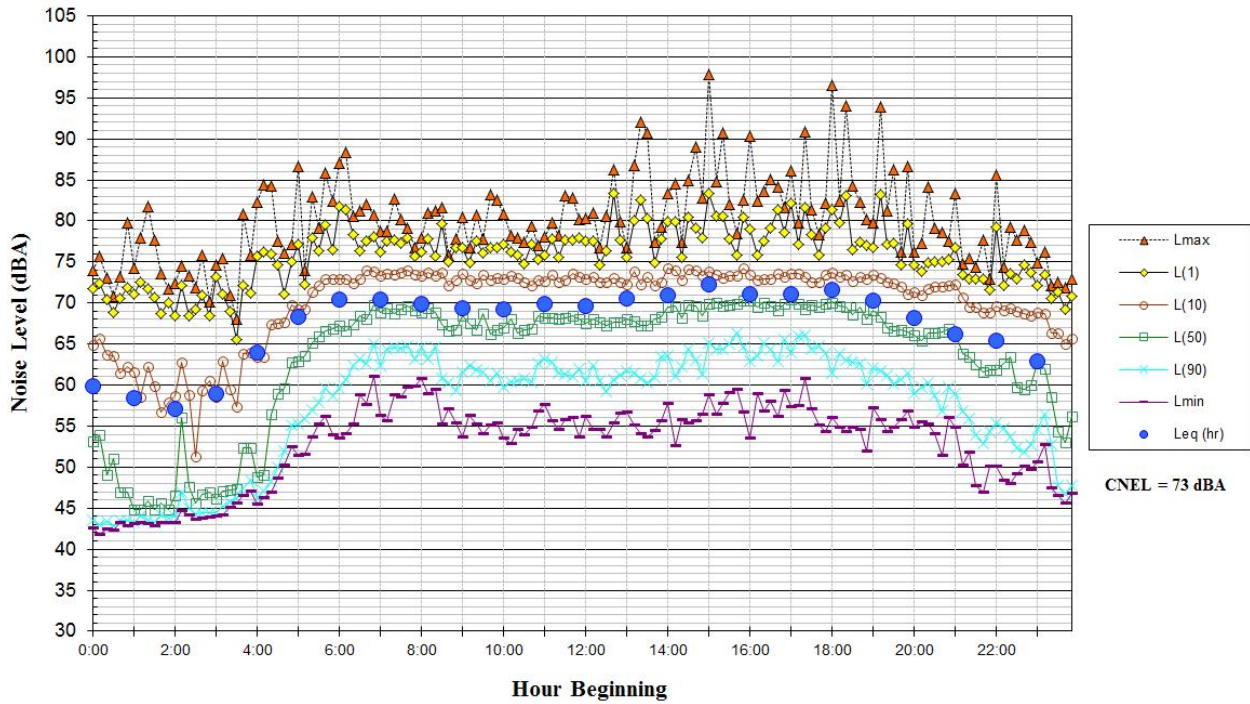
Noise Levels at Noise Measurement Site LT-3 Along Northeast Property Line, ~50 Feet South of Coleman Ave Centerline Friday, March 17, 2017
