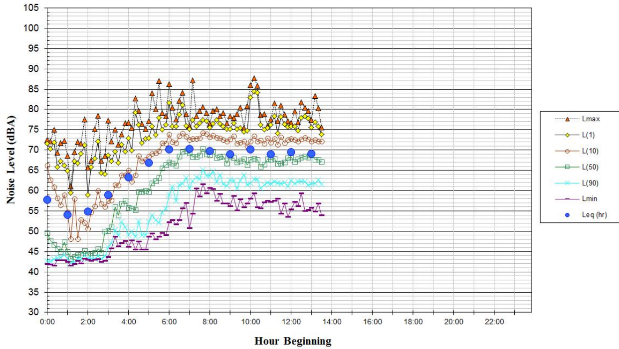
Noise Levels at Noise Measurement Site LT-3 Along Northeast Property Line, ~50 Feet South of Coleman Ave Centerline Monday, March 20, 2017
