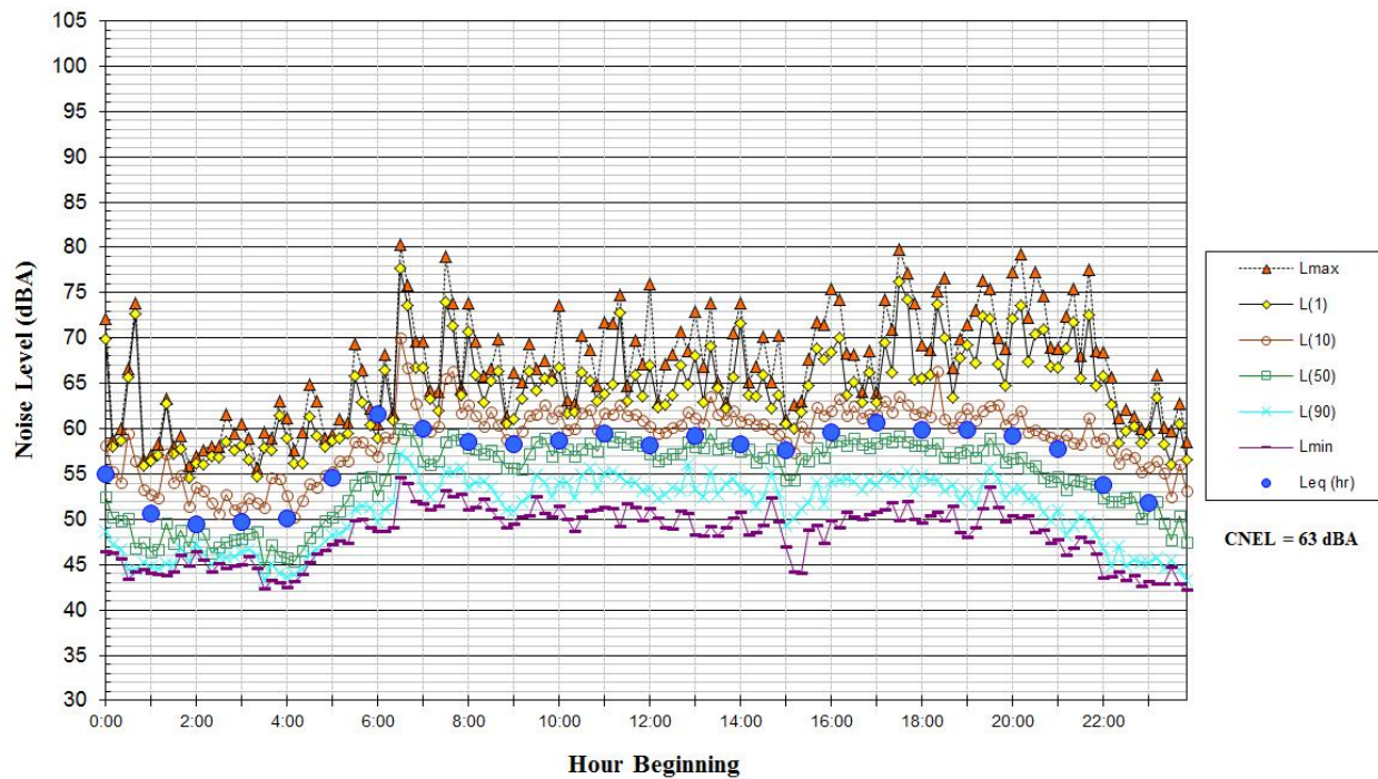
Noise Levels at Noise Measurement Site LT-2 Along Southeast Property Line, ~290 Feet Southwest of Coleman Ave Centerline Saturday, March 18, 2017
