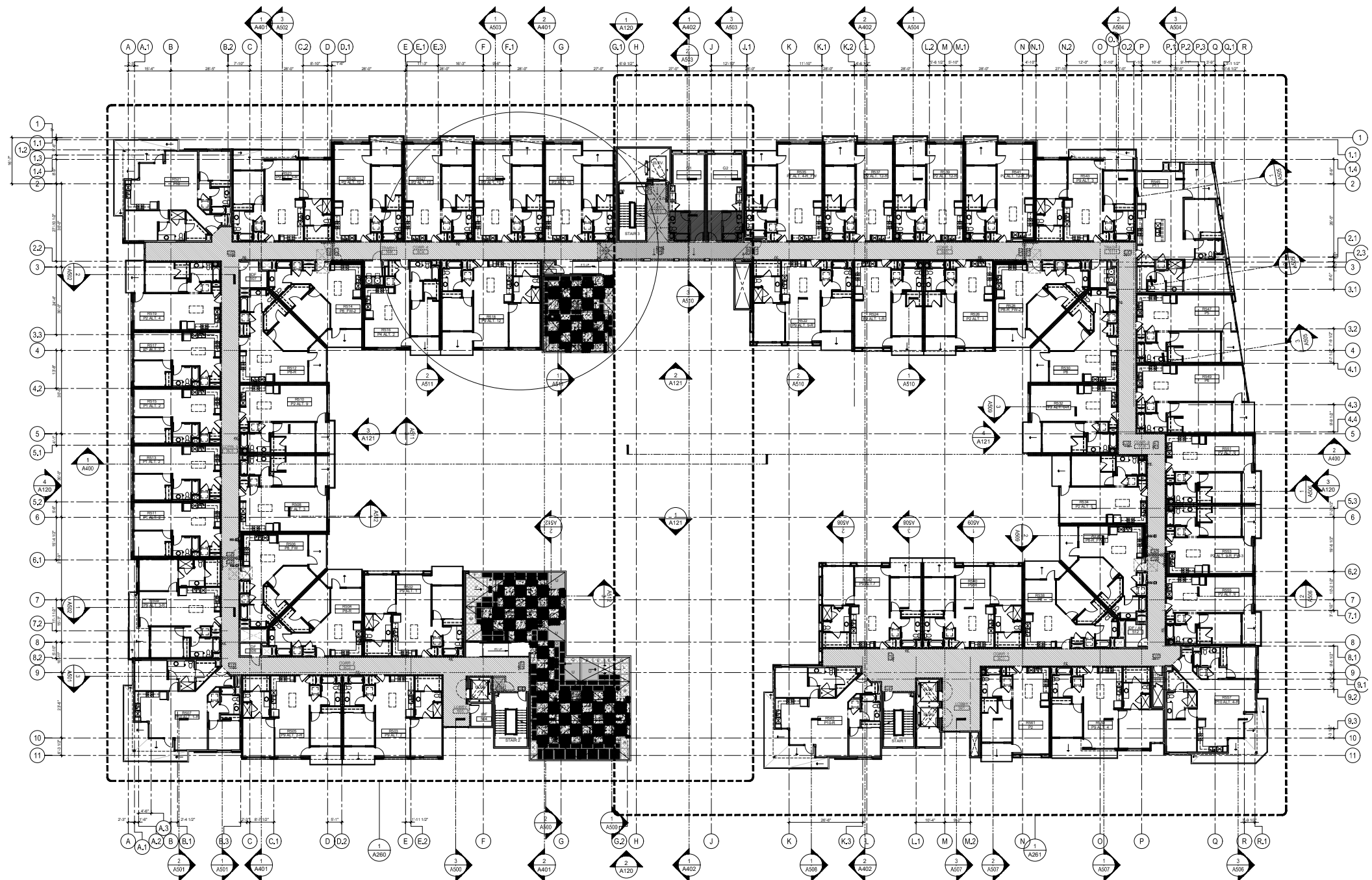
LAWRENCE STATION - BUILDING A R5 FLOOR PLAN
