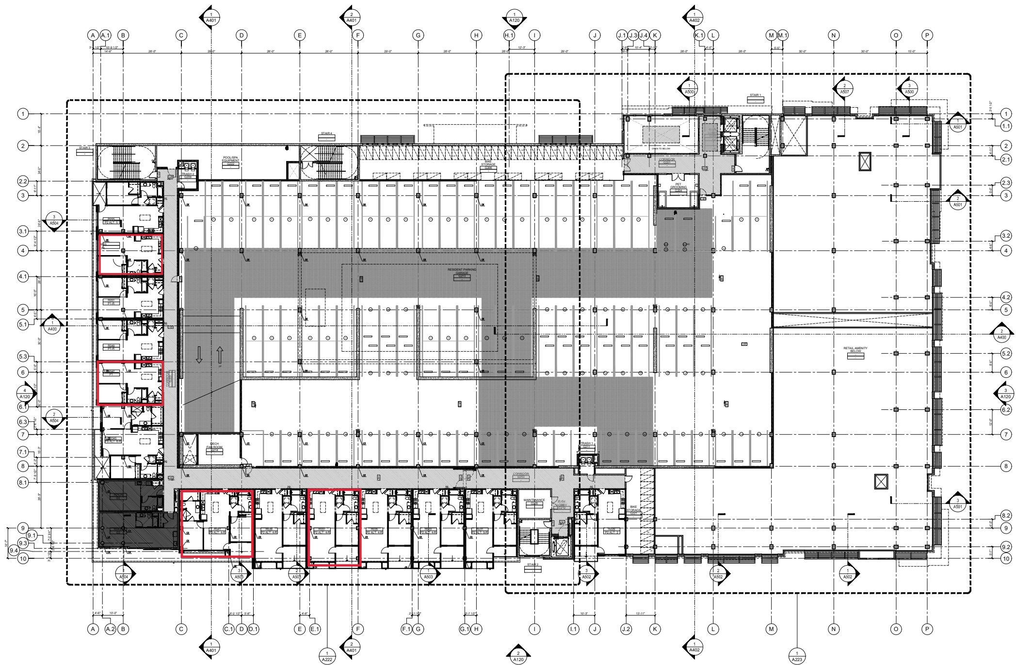
LAWRENCE STATION - BUILDING B G2 FLOOR PLAN
